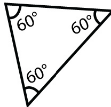
Equiangular Triangle
