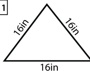
Equilateral Triangle
