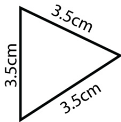
Equiangular Triangle
