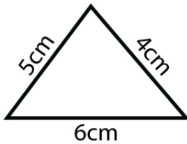
Scalene Triangle
