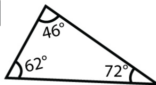
Acute Triangle
