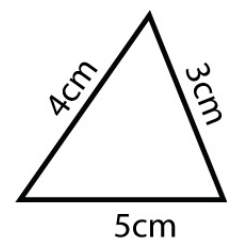
Scalene Triangle
