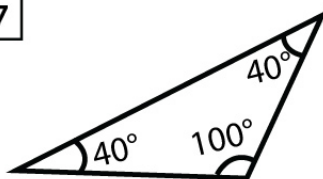
Obtuse Triangle
