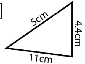
Scalene Triangle
