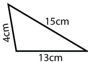
Scalene Triangle
