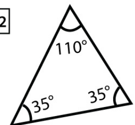
Obtuse Triangle
