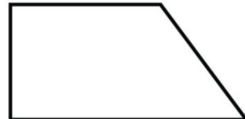
Trapezoid
