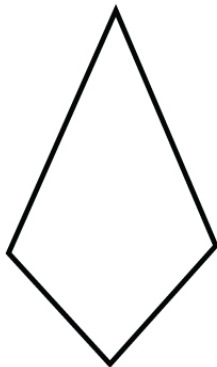
Kite
